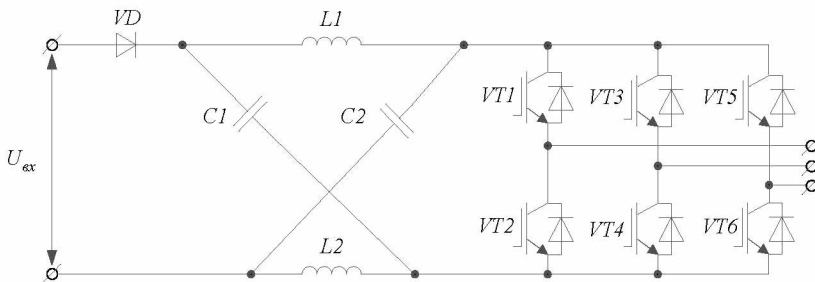
Fig. 2. Block diagram of the z-inverter
