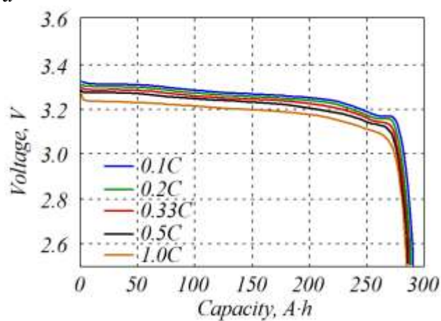
Fig. 2. Charge-discharge characteristics: a – lithium-ion battery LIR18650; b – lithium-iron-phosphate battery LF280
