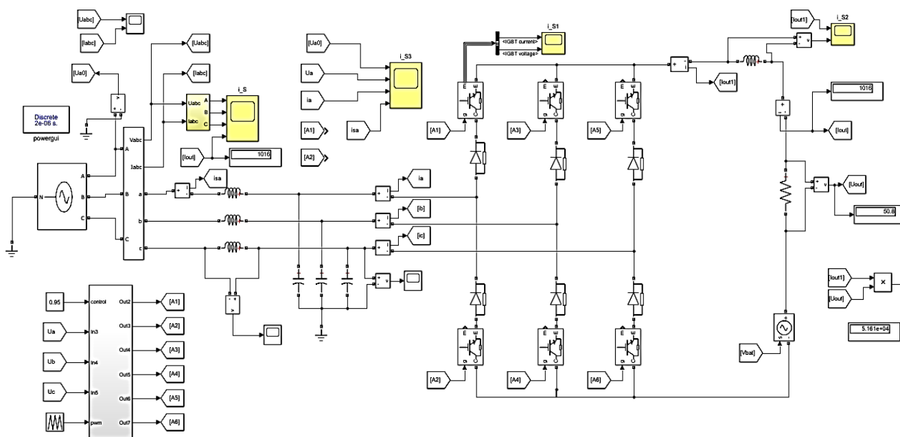
Fig. 2. Model of an electric vehicle charging station based on the CSR
