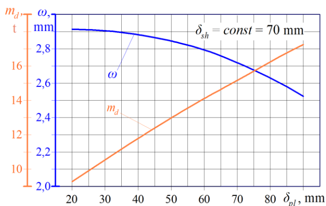
Fig. 3. Relationship between plate flexure \omega , drum's mass m_d , and plate's thickness \delta_{pl}
